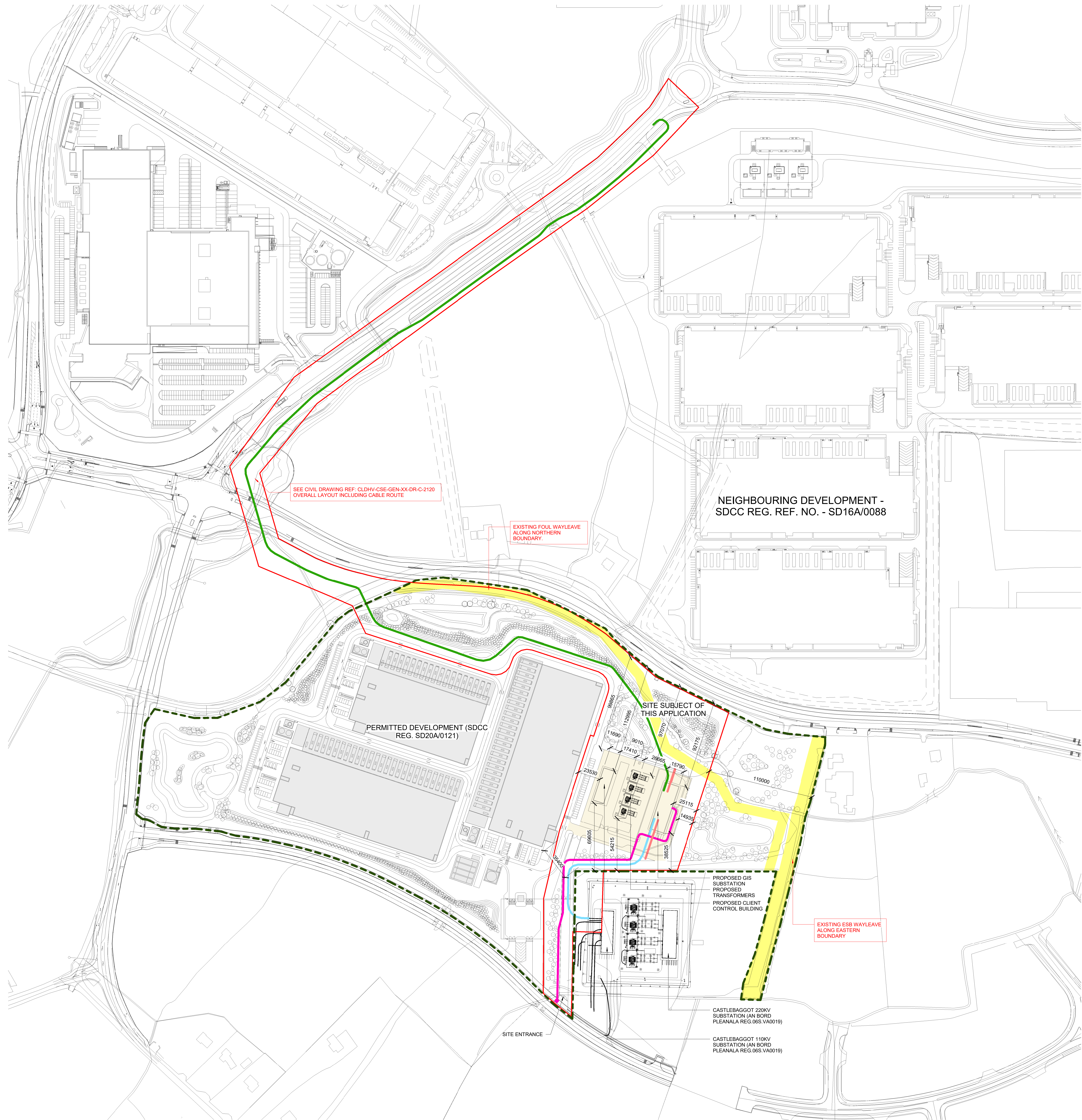
1 PROPOSED SITE LAYOUT PLAN 1 : 1500
